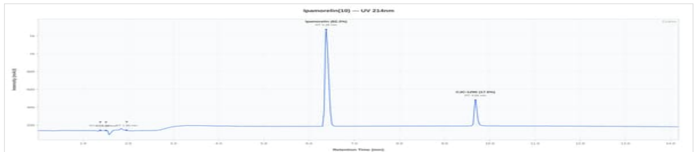
CJC-1295 / Ipamorelin 10 - PL-CIP10-S52-G03: UV Chromatogram
