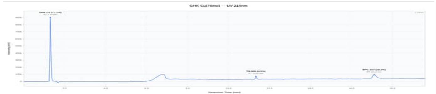
GLOW 70mg - PL-GL70-S52-G03: UV Chromatogram
